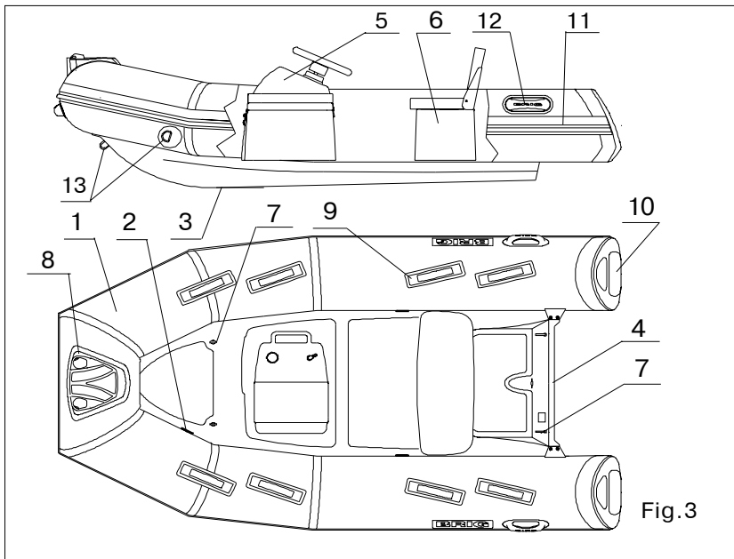
TENDER DELUXE version Boat General View (see Fig.3).
