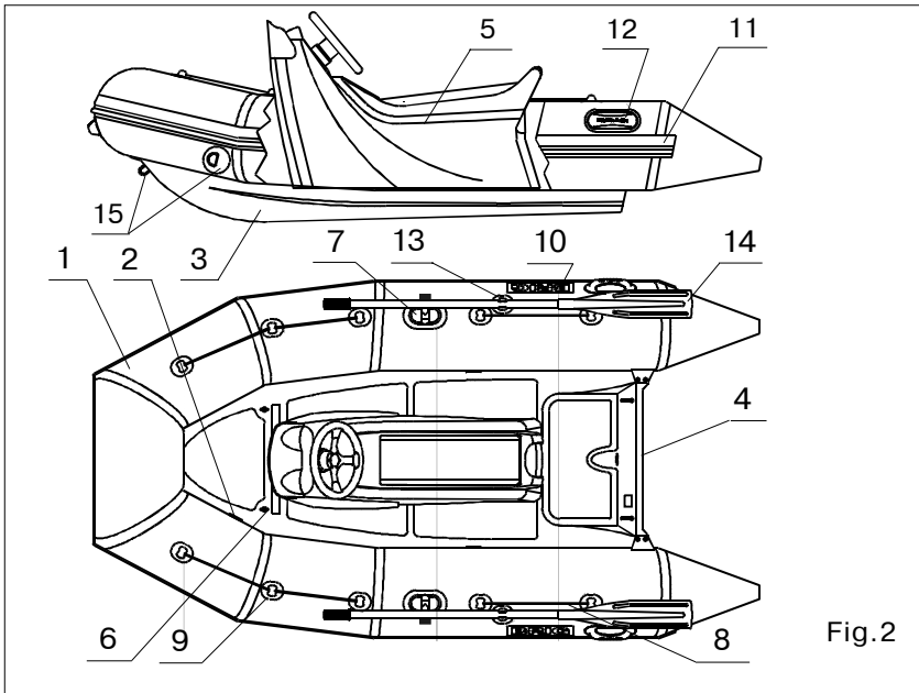
SPORT version Boat General View (see Fig.2).
